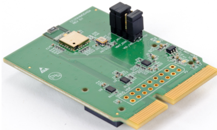
Figure 6-15. CC2564MODAEM Board
