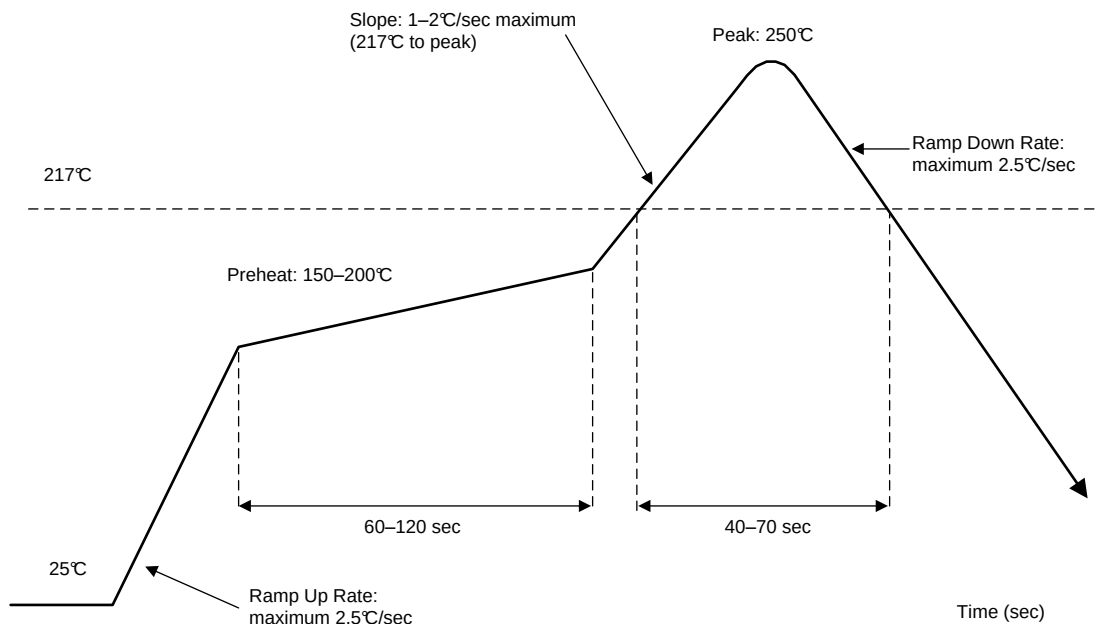
Figure 6-16. Reflow Profile
