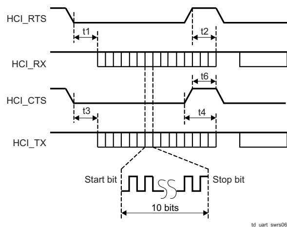
Figure 4-2. UART Timing
