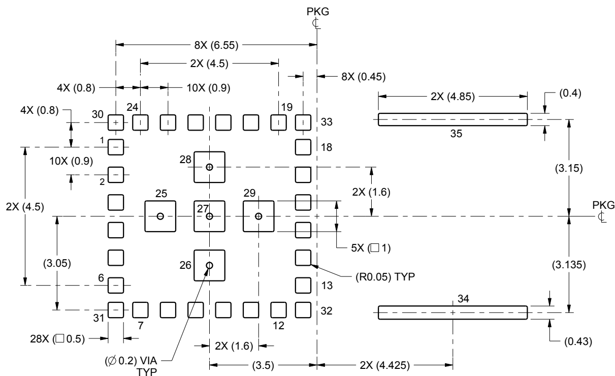
LAND PATTERN EXAMPLE SCALE:8X
