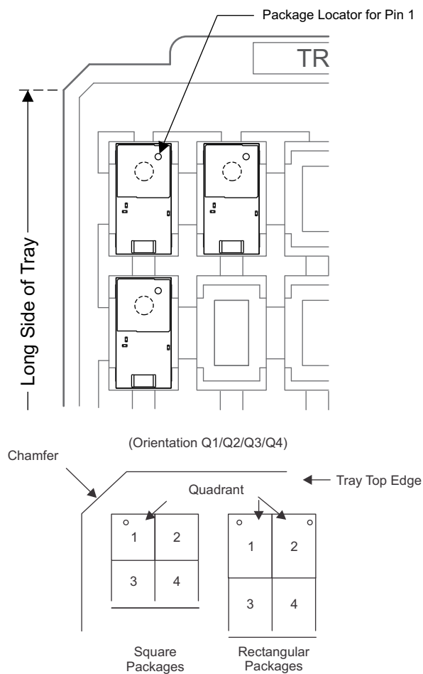
Figure 8-16. Pin 1 Orientation in Tray
