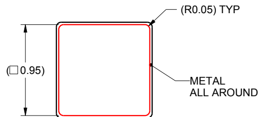
PAD DETAIL 4X, SCALE:25X
